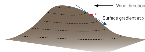
Figure 6.6 Exposure transformation
